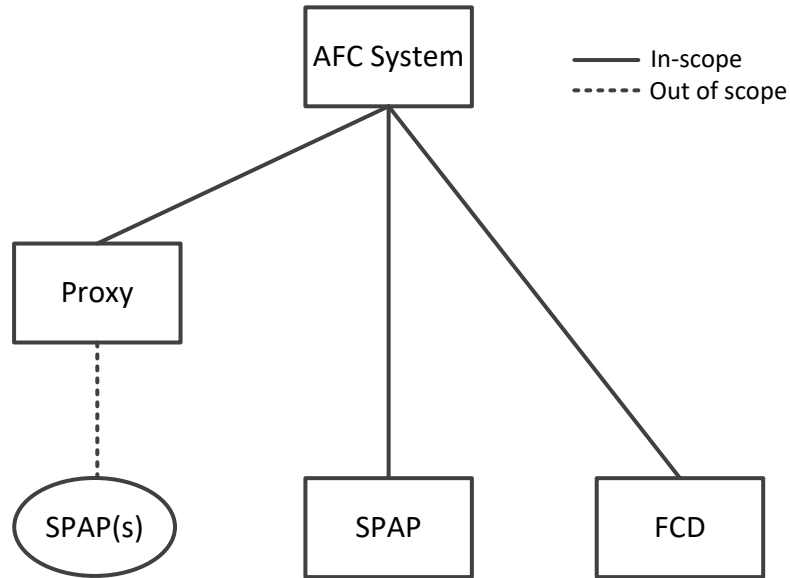
Figure 1: Protocol Interface
