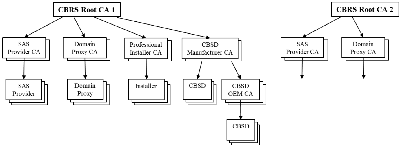
Figure 1: PKI Structure
