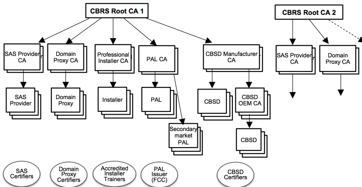
Figure 1: PKI Structure
