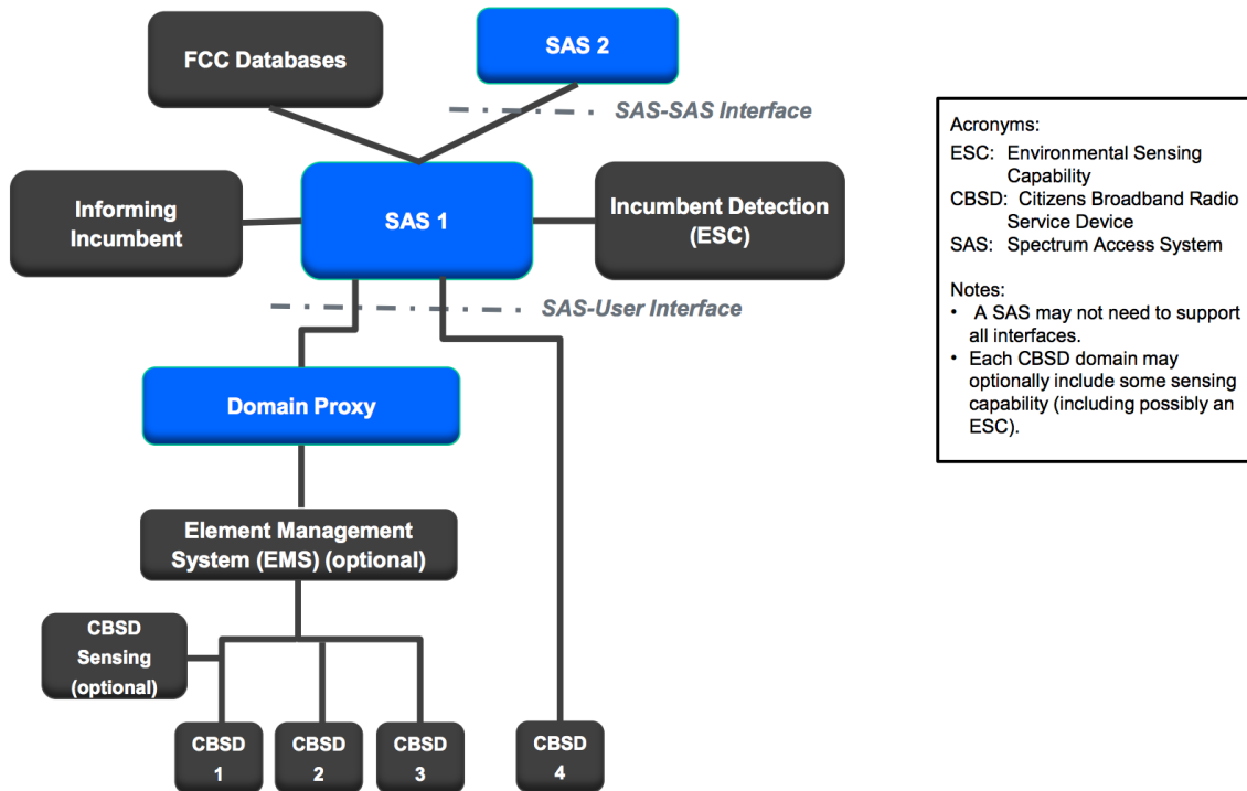
Figure 1. SAS Notional Architecture
