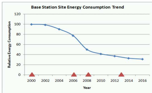
Figure 3 – Improvements in the energy consumption of different versions of base station equipment (assuming same configuration and operation). Markers identify the years of the releases assumed in this study.
