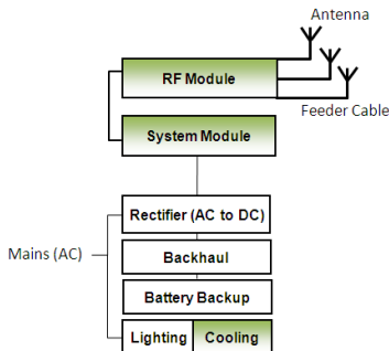
Figure 1 – Modular overview of some of the main components in a typical macro base station.
