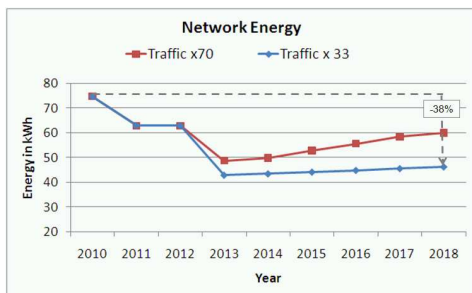
Figure 7 – Overview of the energy trend for both traffic growth cases while assuming a full equipment replacement strategy (best case scenario)
