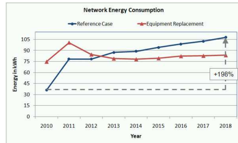
Figure 5 – An overview of how the energy consumption develops for the two cases. This graph is represents the case with an aggressive traffic growth.
