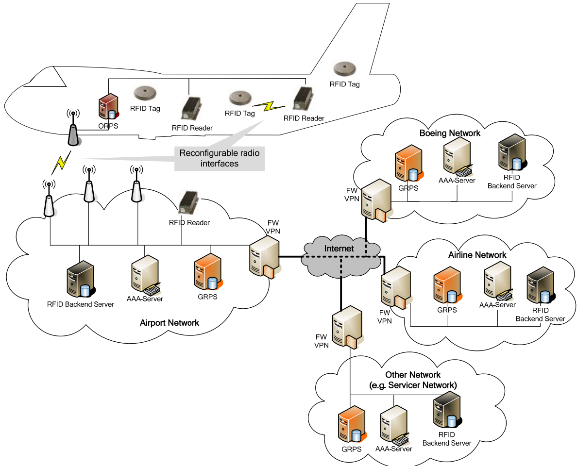
Figure 1: Mobile Multi-Purpose RFID System SDR Forum Technical Conference 2007
